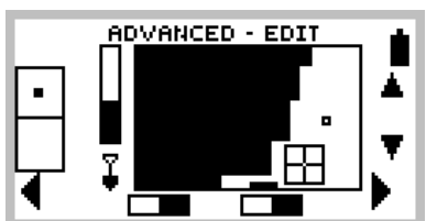
Figure 6.9 Edit screen
